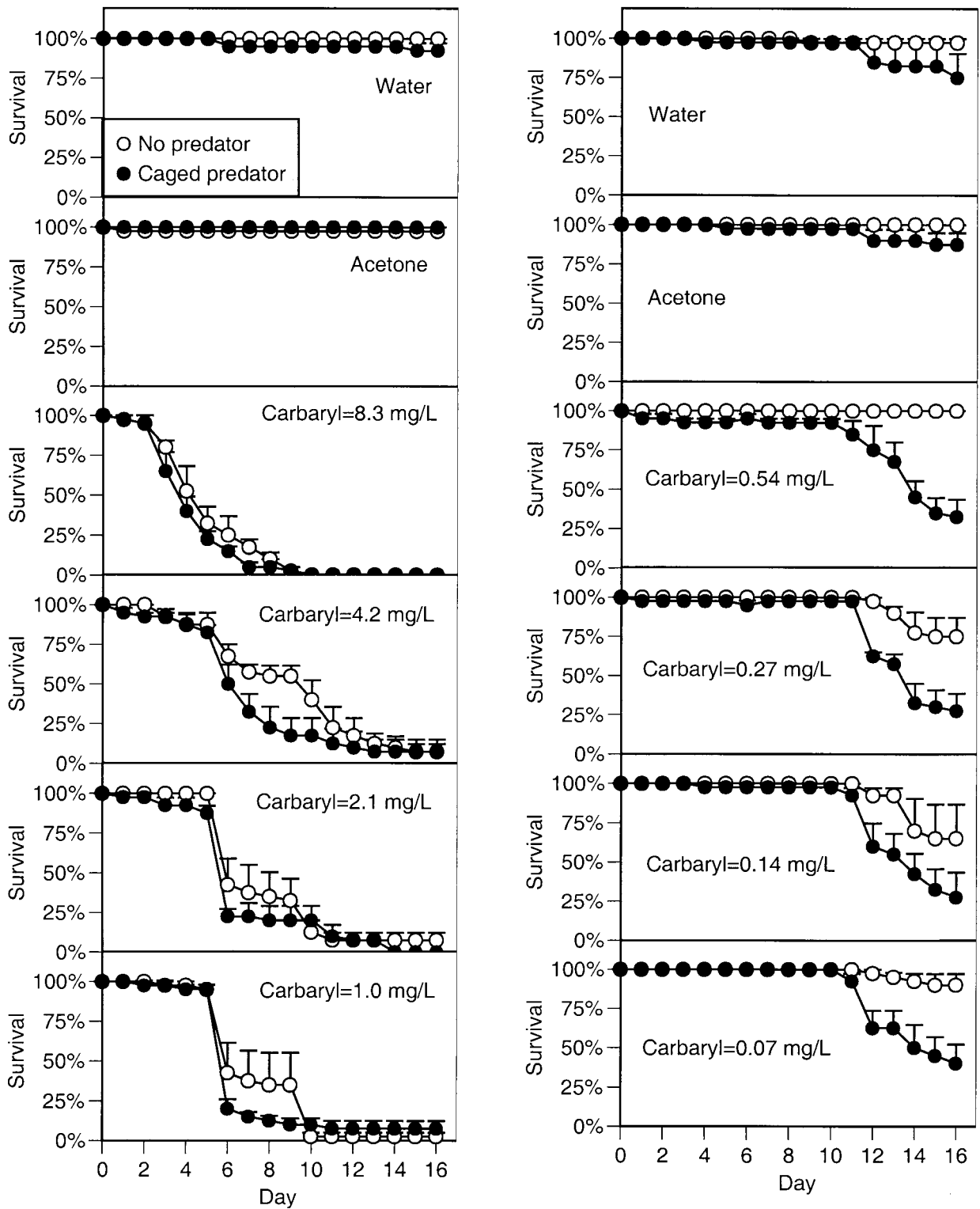
Fig. 3. Survivorship of gray treefrog tadpoles reared in the presence or absence of predatory cues combined with the addition of water (a negative control), acetone (a solvent control), or carbaryl at eight concentrations (experiments 2 and 3). Data are means \pm 1 SE. (Left) Experiment 2. (Right) Experiment 3.
