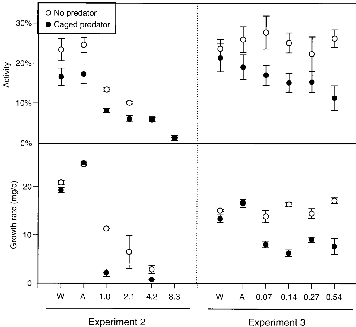
Fig. 2. Activity and growth rate of gray treefrog tadpoles reared in the presence or absence of predatory cues combined with the addition of water (W; a negative control), acetone (A; a solvent control), or carbaryl (numbers along the x axis represent carbaryl concentrations in mg/liter). Data are means \pm 1 SE (experiments 2 and 3).
