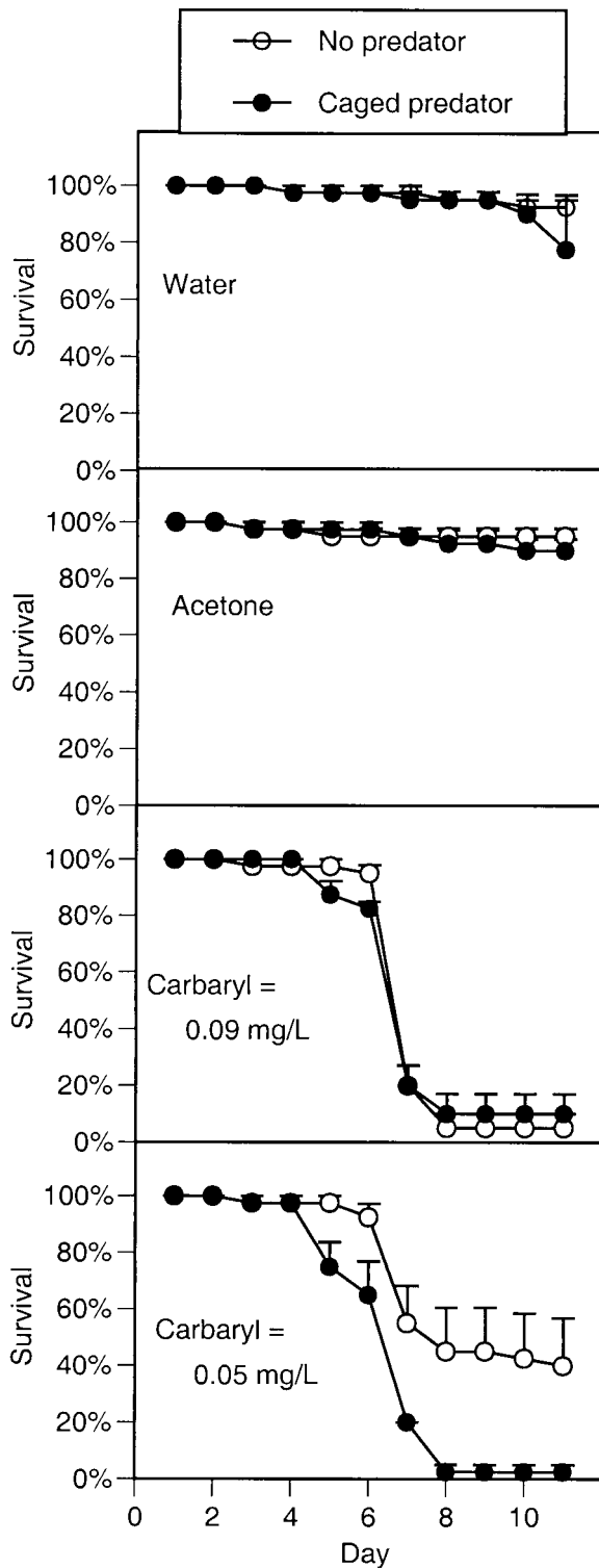
Fig. 1. Survivorship of gray treefrog tadpoles reared in the presence or absence of predatory cues combined with the addition of either water (a negative control), acetone (a solvent control), or two concentrations of carbaryl (experiment 1). Data are means \pm 1 SE.
